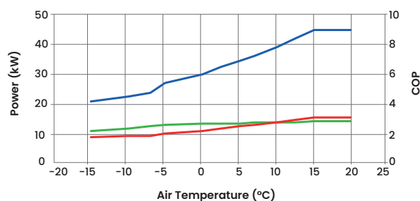
Leeds Performance at 65°C Outlet Temperature
