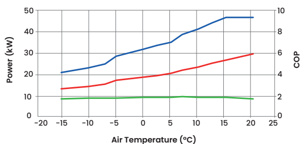
Leeds Performance at 35°C Outlet Temperature
